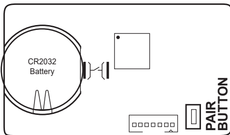
FIGURE 2 TRX Transceiver Circuit Board
