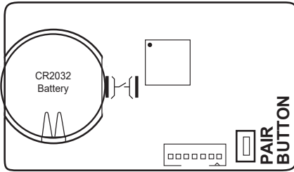
FIGURE 2 TRX Transceiver Circuit Board
