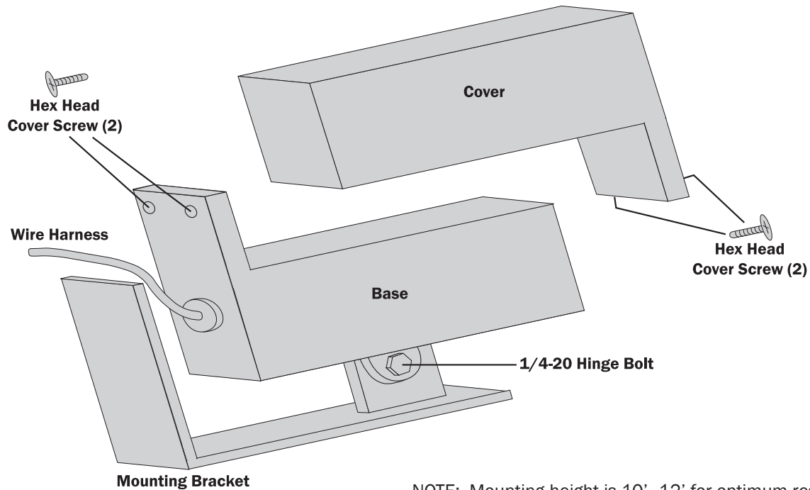
FIGURE 1a SmartWalk XP Housing
