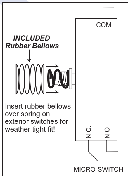
BELLOWS DIAGRAM
