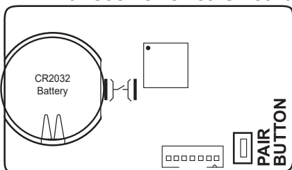
FIGURE 2 TRX Transceiver Circuit Board
