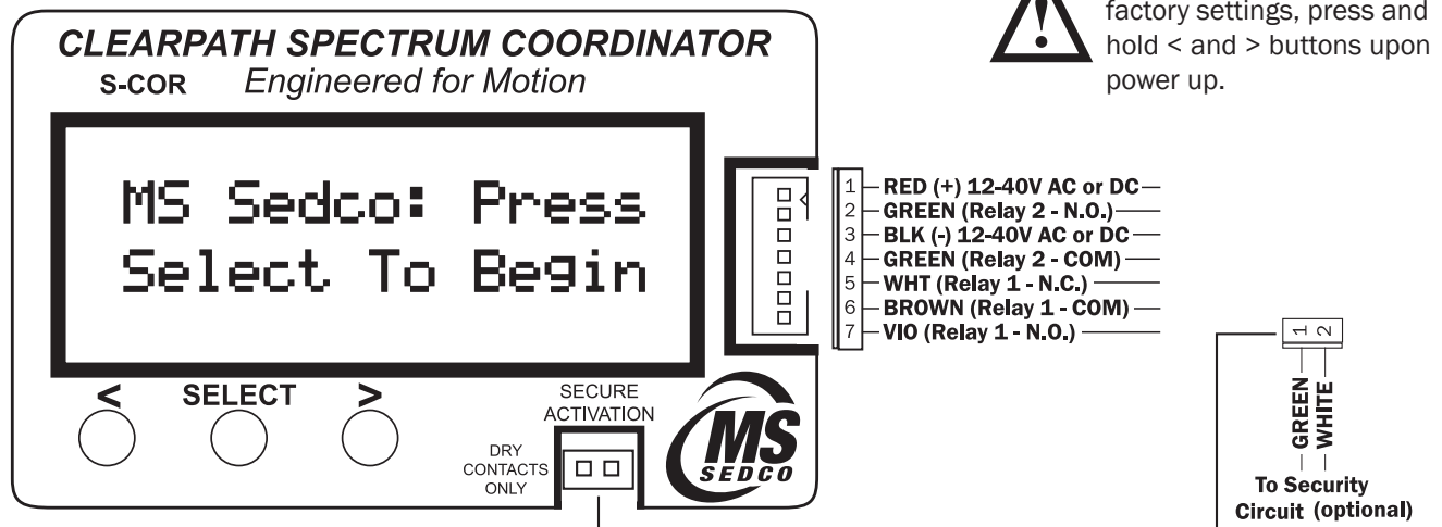
FIGURE 1 Wiring Diagram
